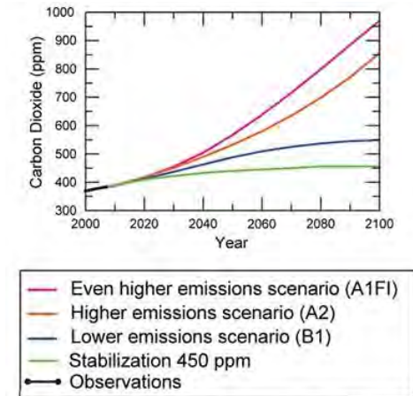
Figure 2. Scenarios for atmospheric carbon dioxide concentration used in a majority of climate models.
